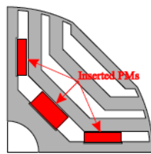
Figure 7. Selected rotor geometry for Case 1 [24]
