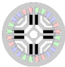
Figure 8. Test motor structure [22]
